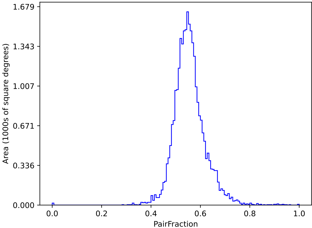
ddf_acor_sf25_lsf40_lsr10_v3.4_10yrs (g or r or i): PairFraction
