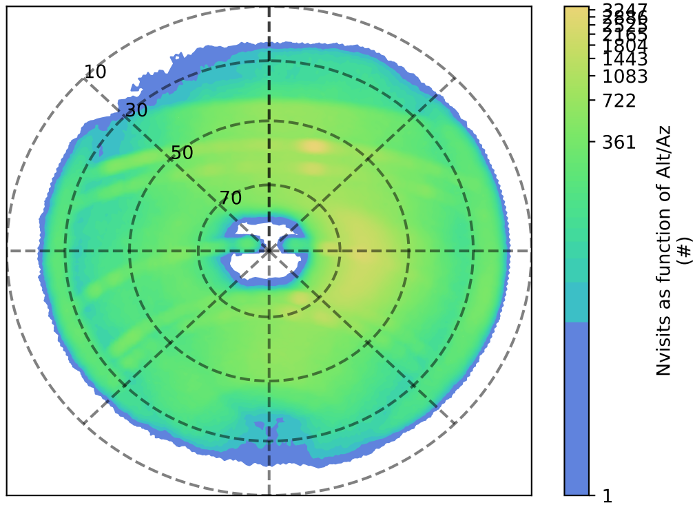
ddf_acor_sf25_lsf40_lsr10_v3.4_10yrs z: Nvisits as function of Alt/Az
