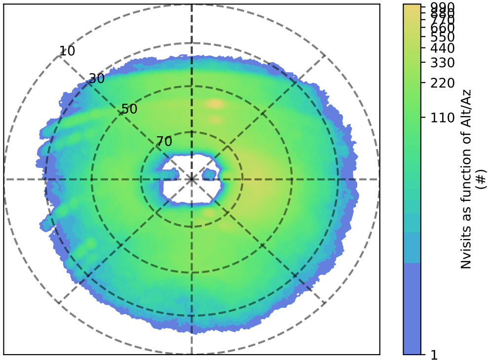
ddf_acor_sf25_lsf40_lsr10_v3.4_10yrs u: Nvisits as function of Alt/Az
