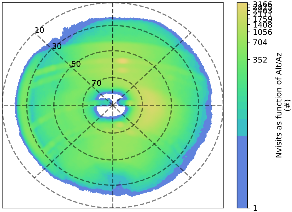
ddf_acor_sf25_lsf40_lsr10_v3.4_10yrs r: Nvisits as function of Alt/Az
