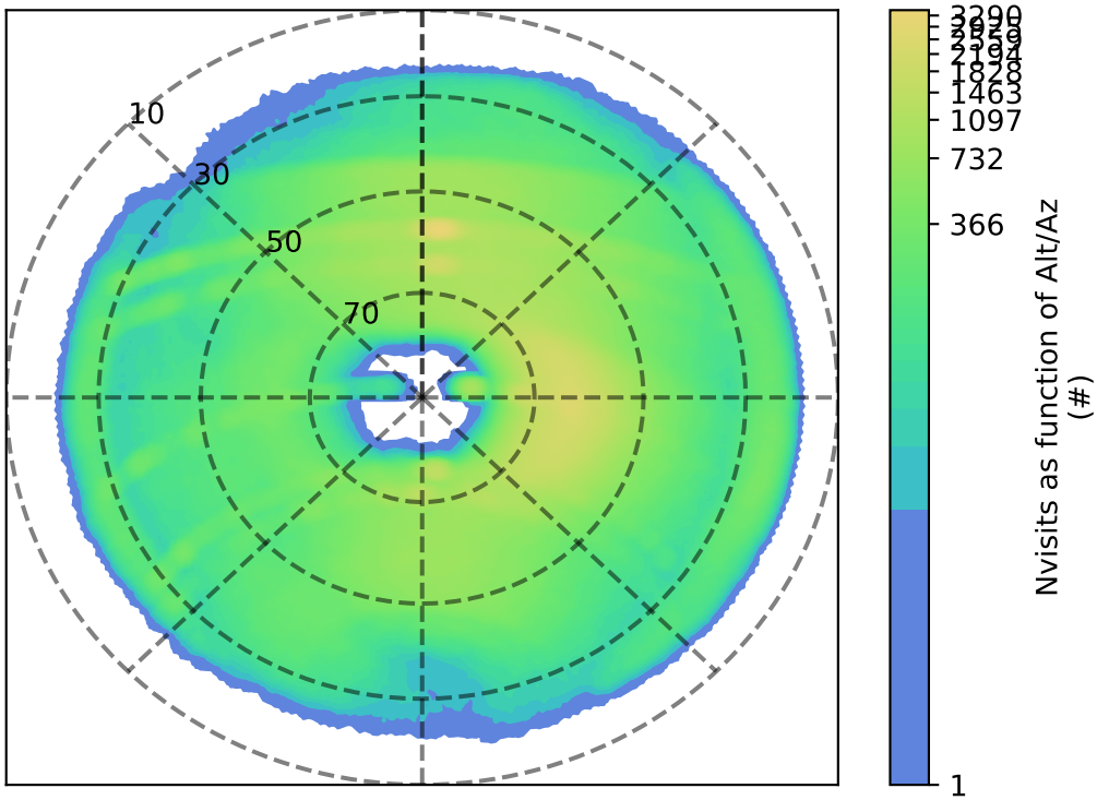
ddf_acor_sf25_lsf40_lsr10_v3.4_10yrs i: Nvisits as function of Alt/Az
