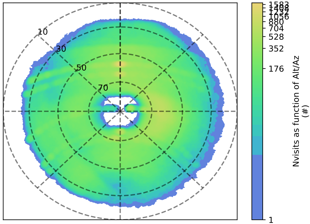
ddf_acor_sf25_lsf40_lsr10_v3.4_10yrs g: Nvisits as function of Alt/Az
