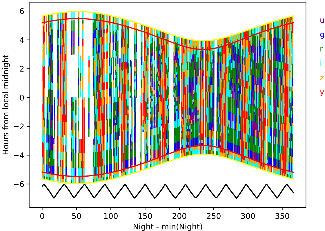
ddf_acor_sf25_lsf40_lsr10_v3.4_10yrs year 9-10: Hourglass
