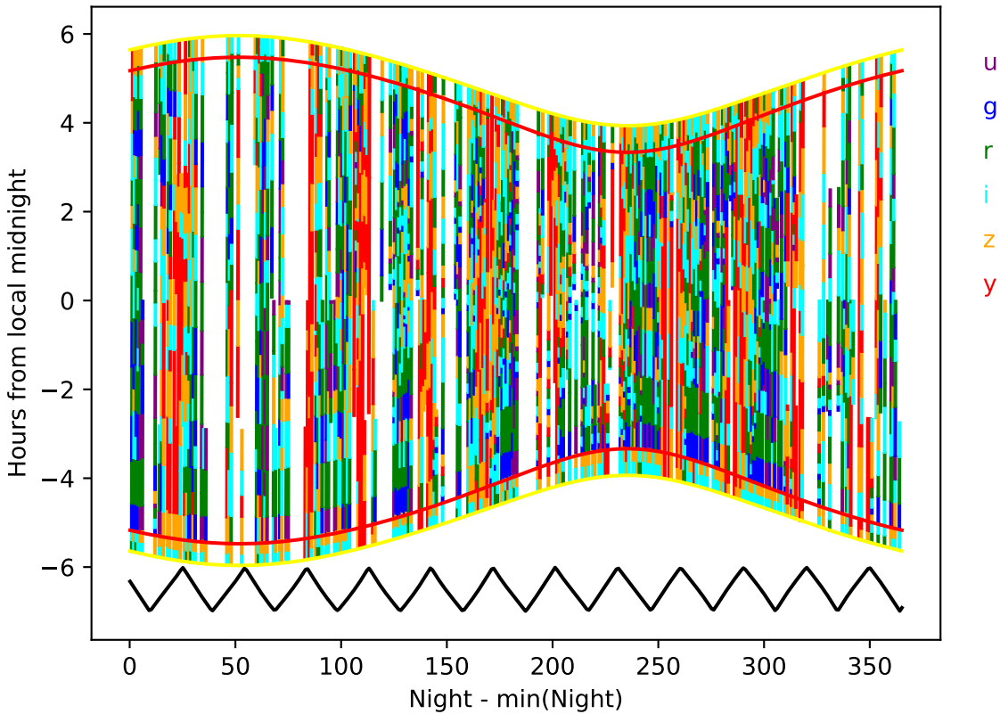
ddf_acor_sf25_lsf40_lsr10_v3.4_10yrs year 7-8: Hourglass
