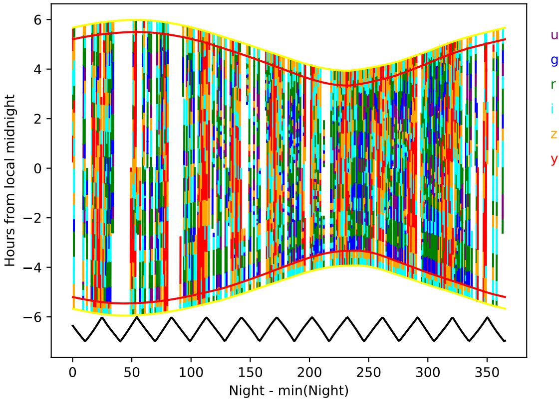
ddf_acor_sf25_lsf40_lsr10_v3.4_10yrs year 4-5: Hourglass
