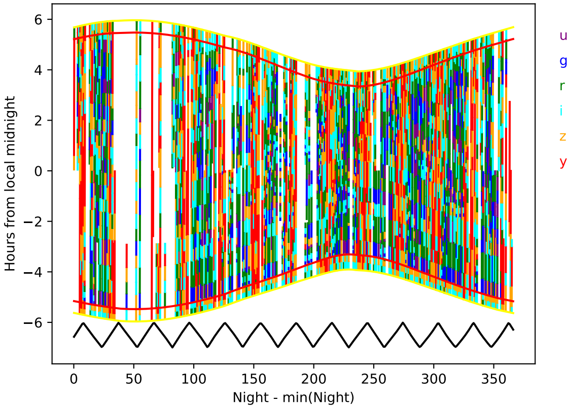
ddf_acor_sf25_lsf40_lsr10_v3.4_10yrs year 3-4: Hourglass
