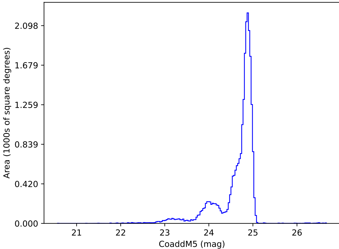
ddf_acor_sf25_lsf40_lsr10_v3.4_10yrs y: CoaddM5
