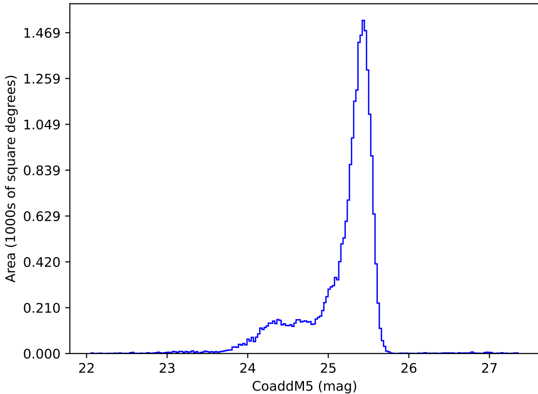
ddf_acor_sf25_lsf40_lsr10_v3.4_10yrs u: CoaddM5
