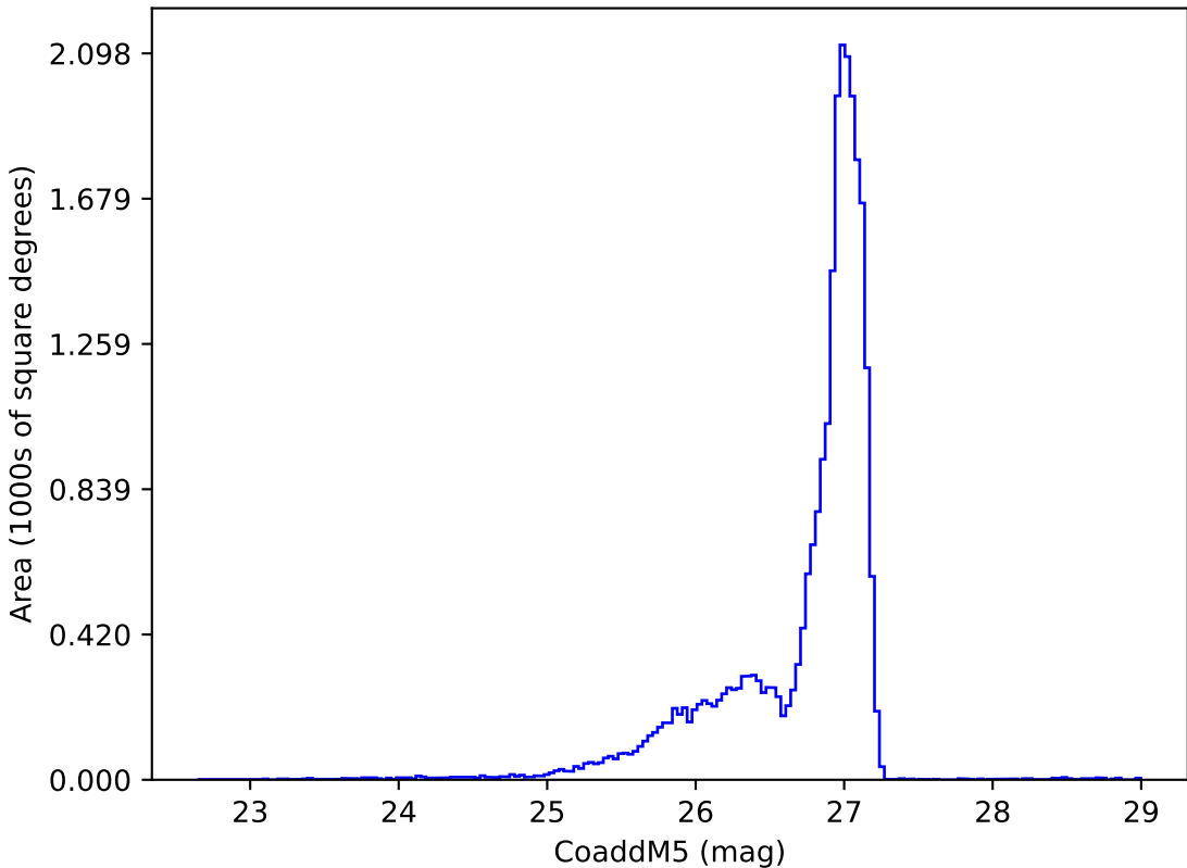
ddf_acor_sf25_lsf40_lsr10_v3.4_10yrs r: CoaddM5
