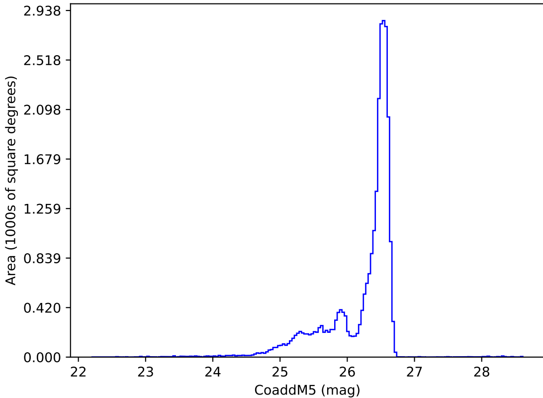
ddf_acor_sf25_lsf40_lsr10_v3.4_10yrs i: CoaddM5
