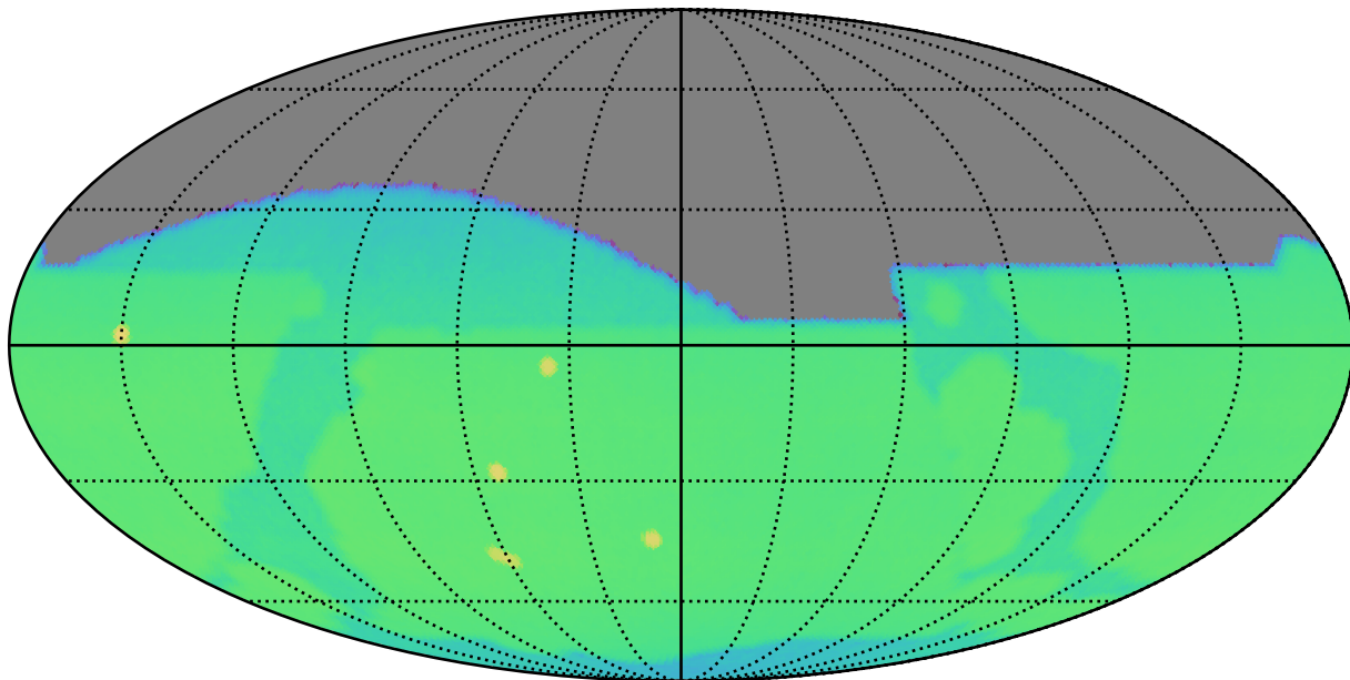
ddf_acor_sf25_lsf40_lsr10_v3.4_10yrs : CoaddM5
