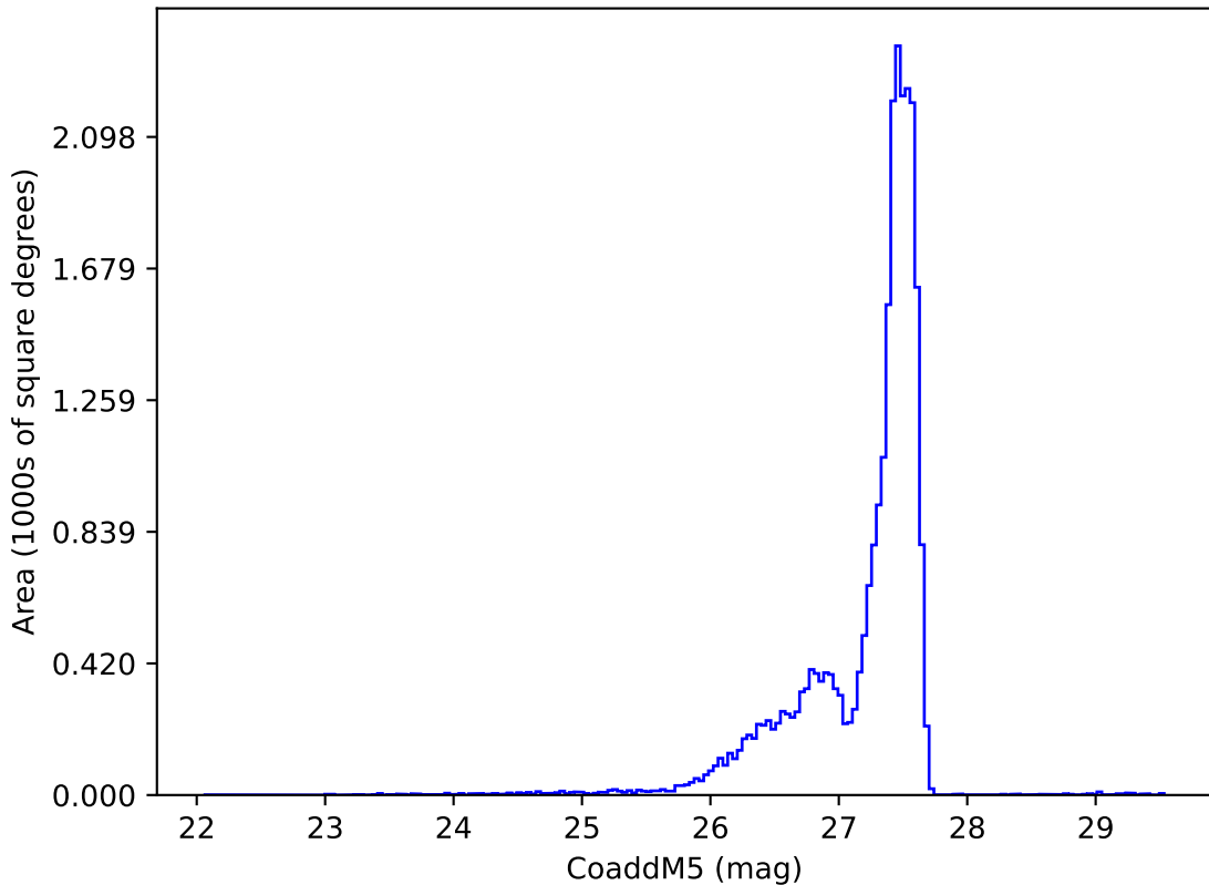
ddf_acor_sf25_lsf40_lsr10_v3.4_10yrs : CoaddM5
