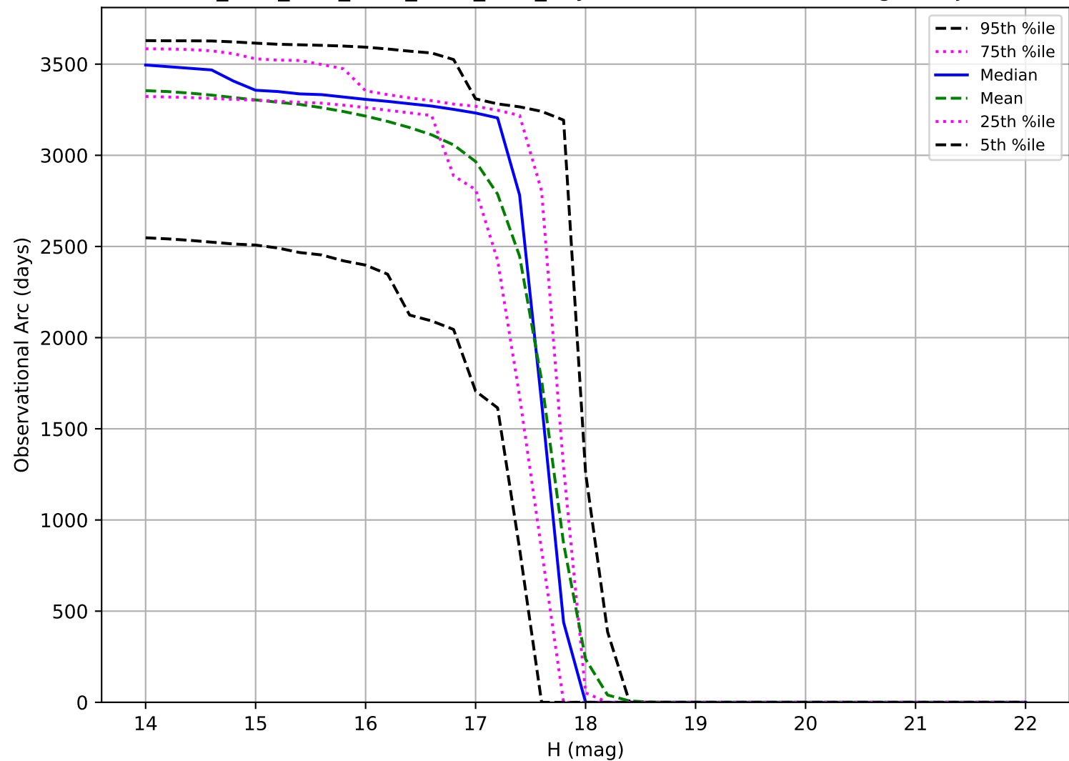
ddf_acor_sf25_lsf30_lsr50_v3.4_10yrs: Observational Arc Length Trojan
