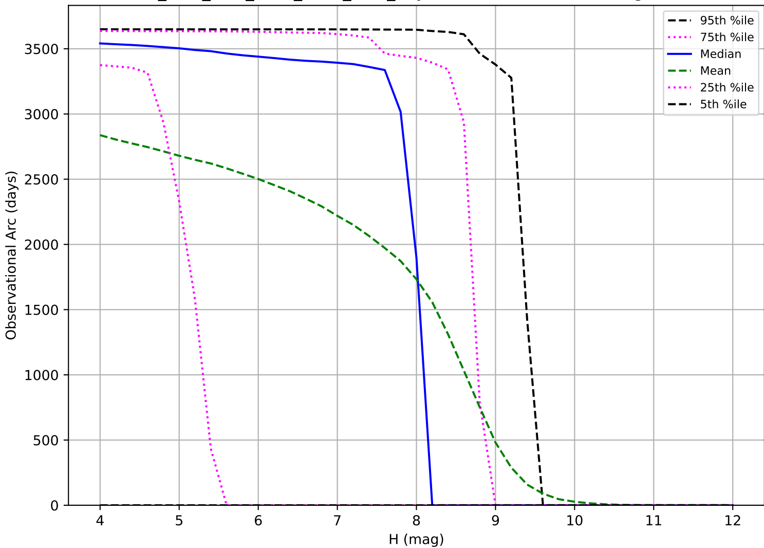
ddf_acor_sf25_lsf30_lsr50_v3.4_10yrs: Observational Arc Length TNO
