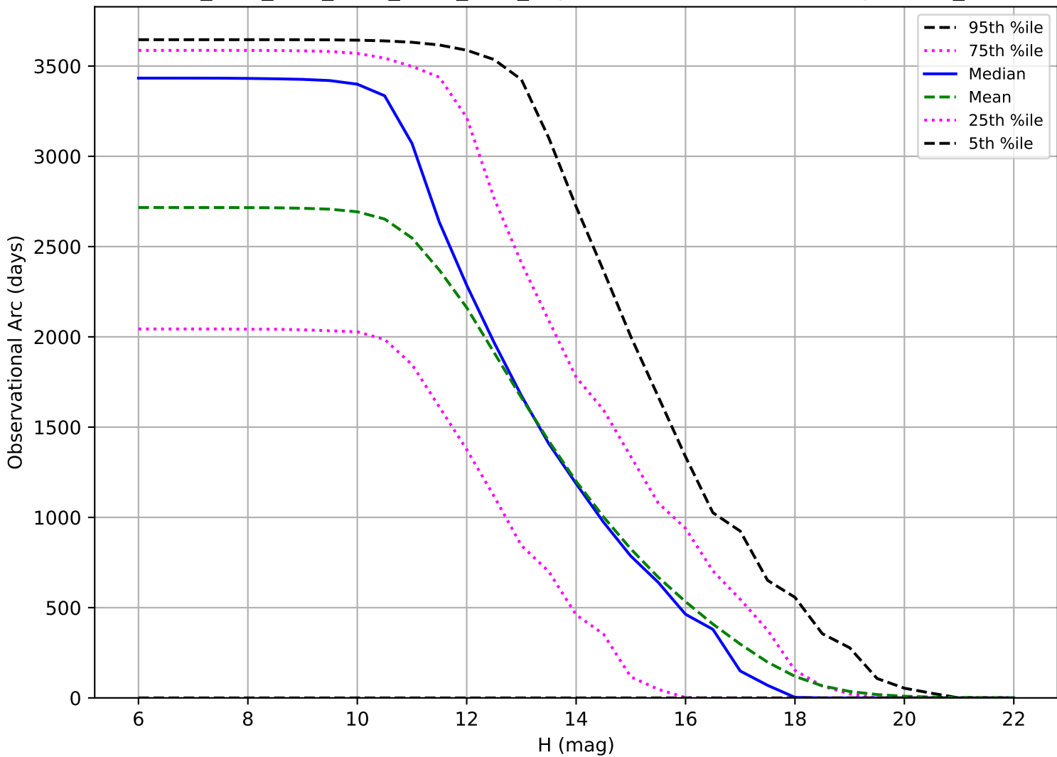
ddf_acor_sf25_lsf30_lsr50_v3.4_10yrs: Observational Arc Length OCC_r5
