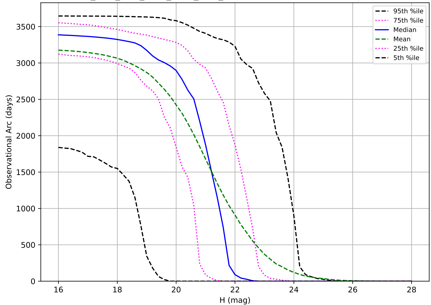
ddf_acor_sf25_lsf30_lsr50_v3.4_10yrs: Observational Arc Length NEO
