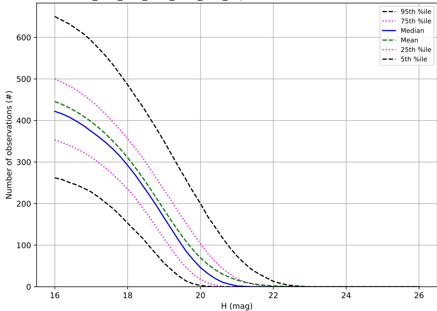
ddf_acor_sf25_lsf30_lsr50_v3.4_10yrs: Number of observations MBA
