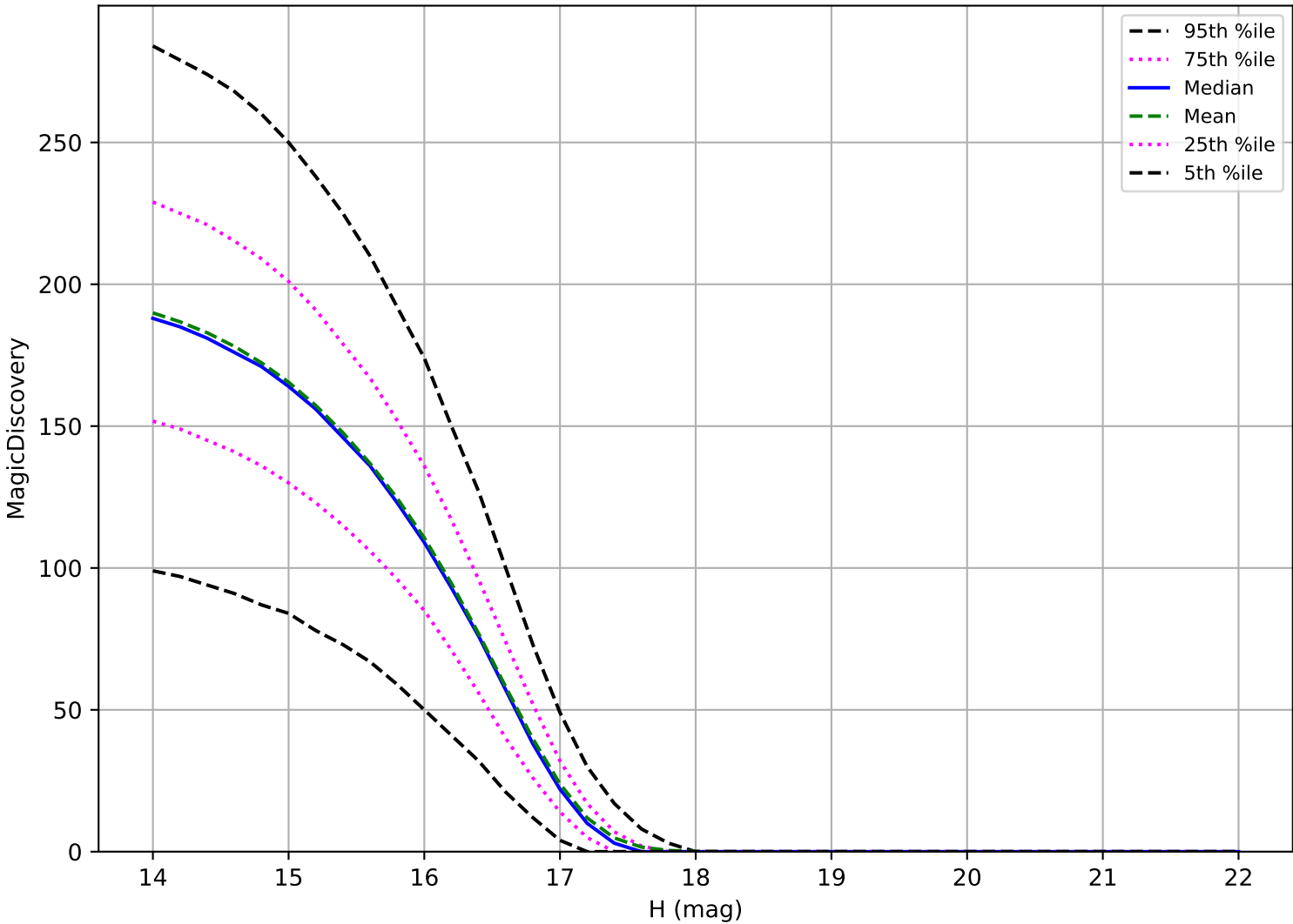
ddf_acor_sf25_lsf30_lsr50_v3.4_10yrs: Trojan 6 detections in 60 nights detection loss
