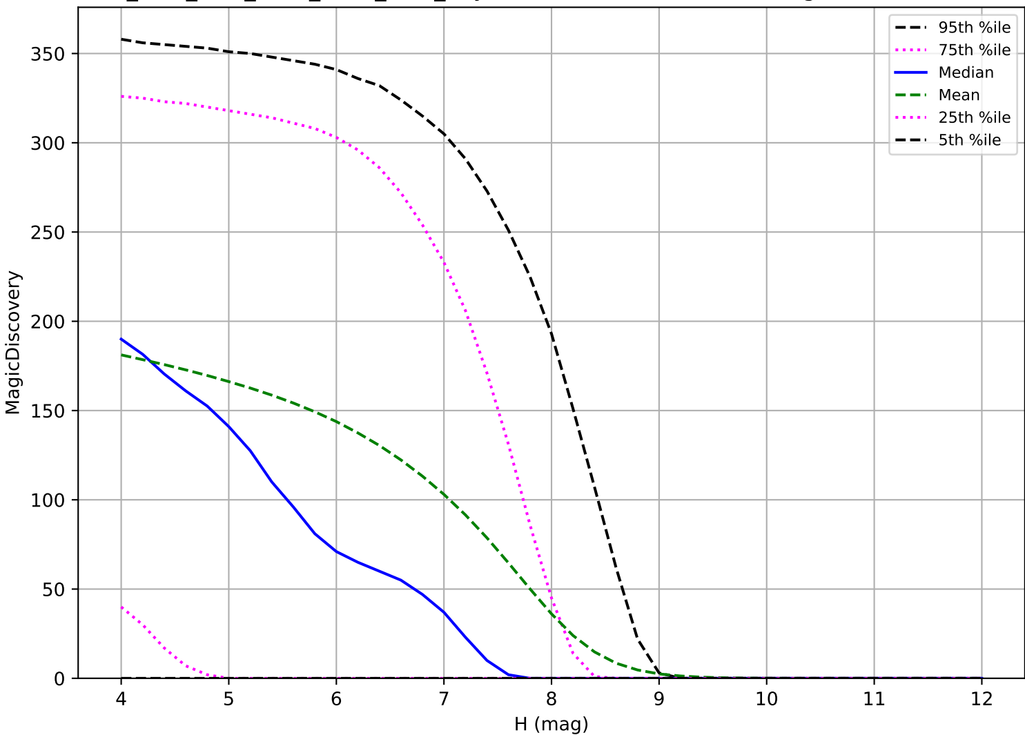
ddf_acor_sf25_lsf30_lsr50_v3.4_10yrs: TNO 6 detections in 60 nights detection loss
