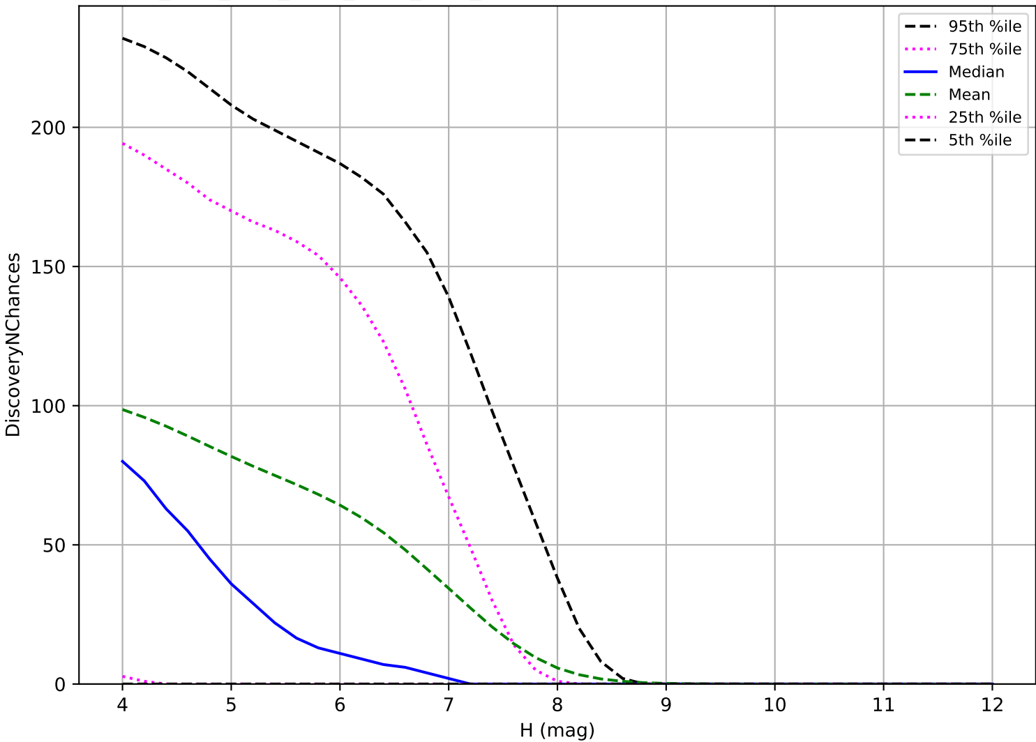
ddf_acor_sf25_lsf30_lsr50_v3.4_10yrs: TNO 3 pairs in 15 nights detection loss
