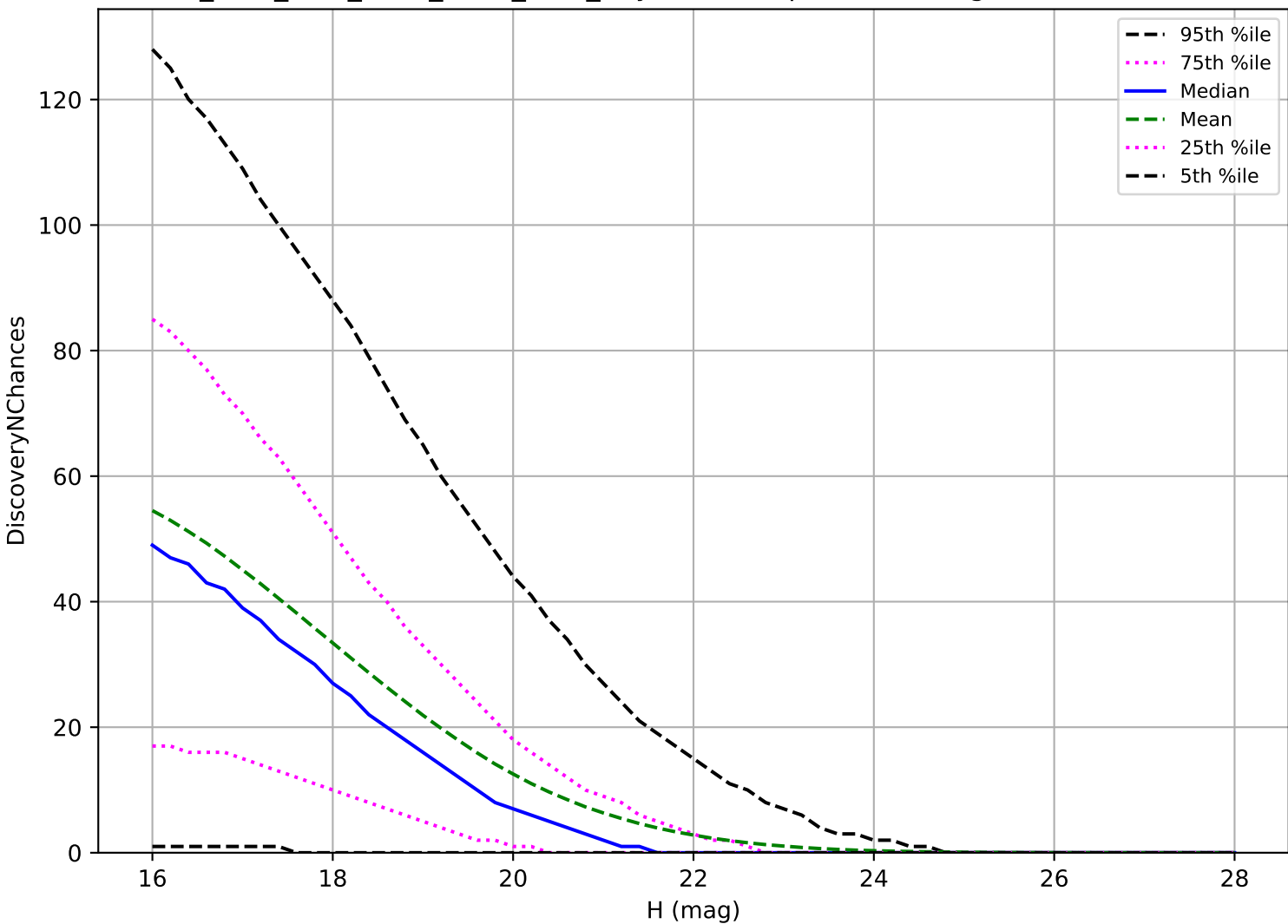
ddf_acor_sf25_lsf30_lsr50_v3.4_10yrs: PHA 3 pairs in 15 nights detection loss
