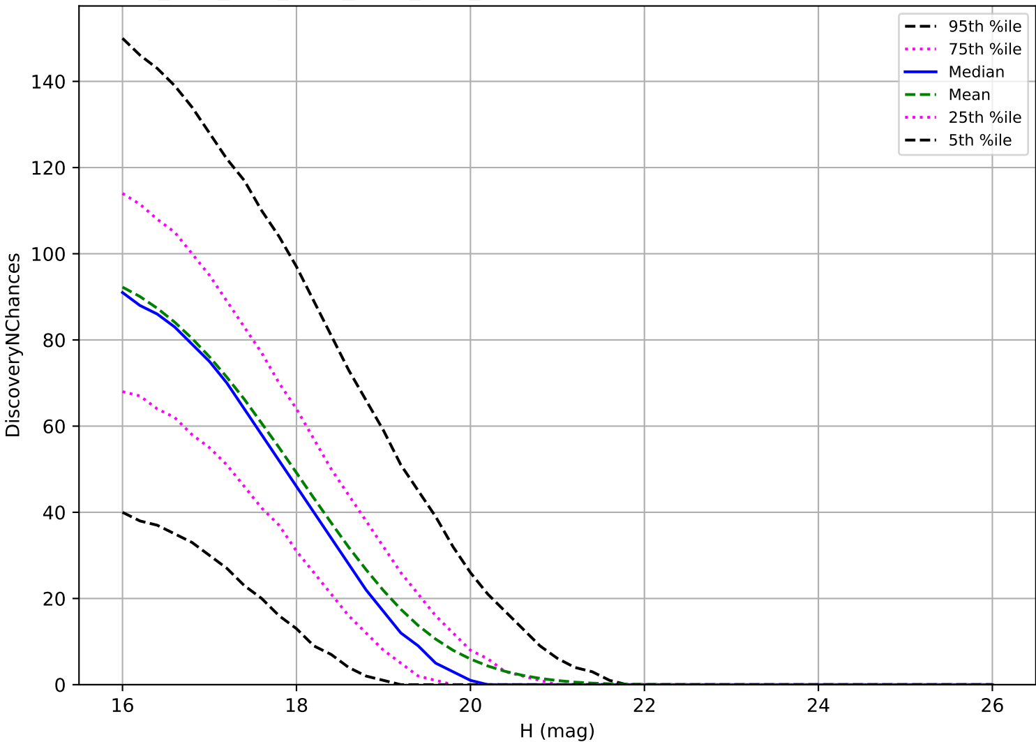
ddf_acor_sf25_lsf30_lsr50_v3.4_10yrs: MBA 3 pairs in 15 nights detection loss
