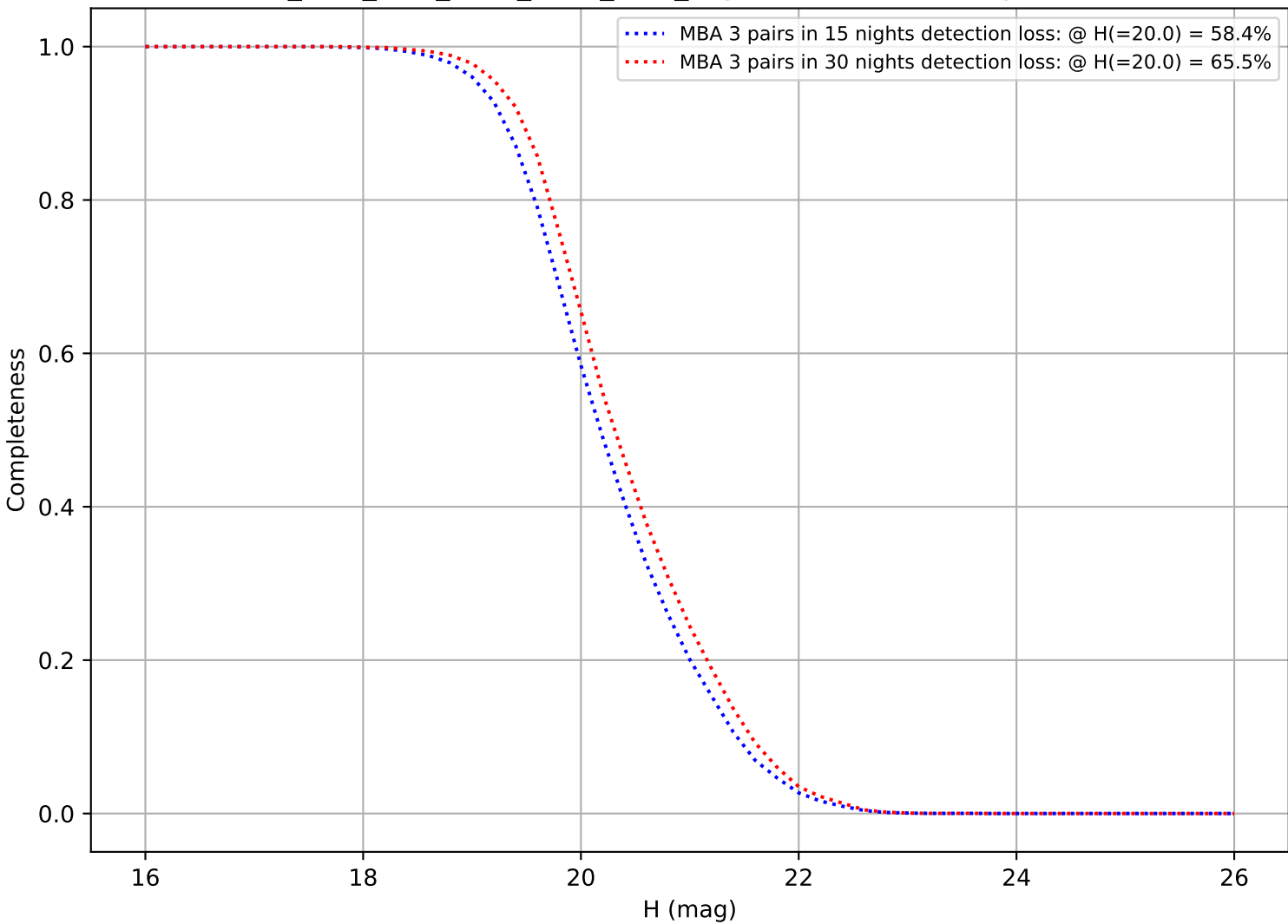
ddf_acor_sf25_lsf30_lsr50_v3.4_10yrs: DifferentialCompleteness
