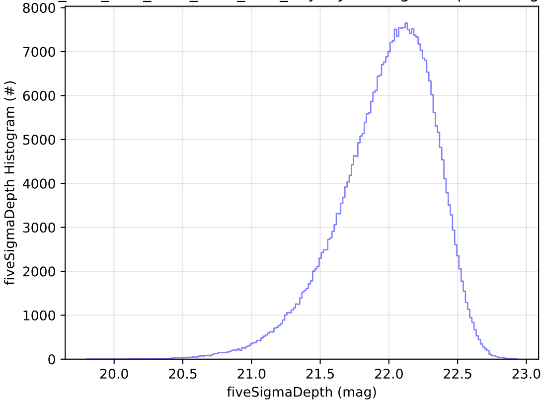
ddf_acor_sf25_lsf30_lsr50_v3.4_10yrs y: fiveSigmaDepth Histogram
