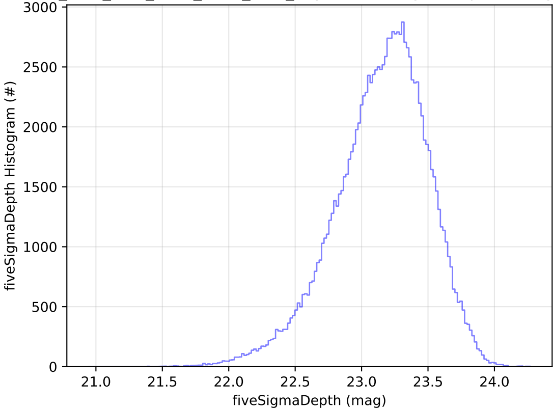
ddf_acor_sf25_lsf30_lsr50_v3.4_10yrs u: fiveSigmaDepth Histogram
