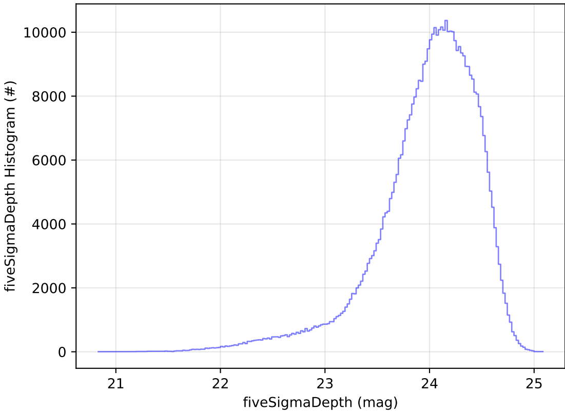
ddf_acor_sf25_lsf30_lsr50_v3.4_10yrs r: fiveSigmaDepth Histogram
