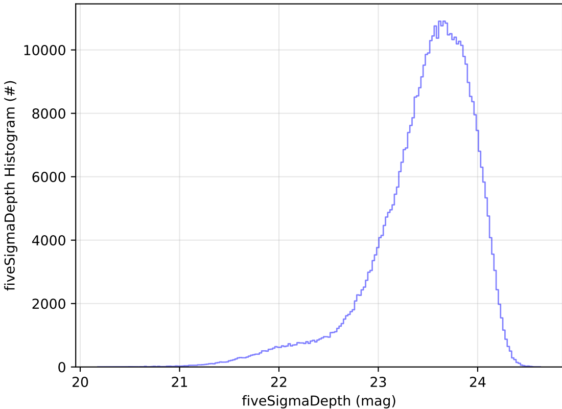
ddf_acor_sf25_lsf30_lsr50_v3.4_10yrs i: fiveSigmaDepth Histogram
