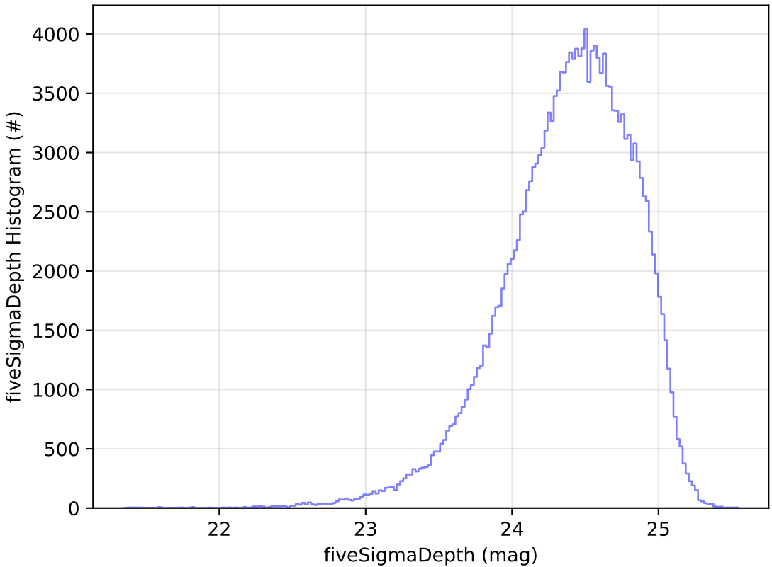
ddf_acor_sf25_lsf30_lsr50_v3.4_10yrs g: fiveSigmaDepth Histogram
