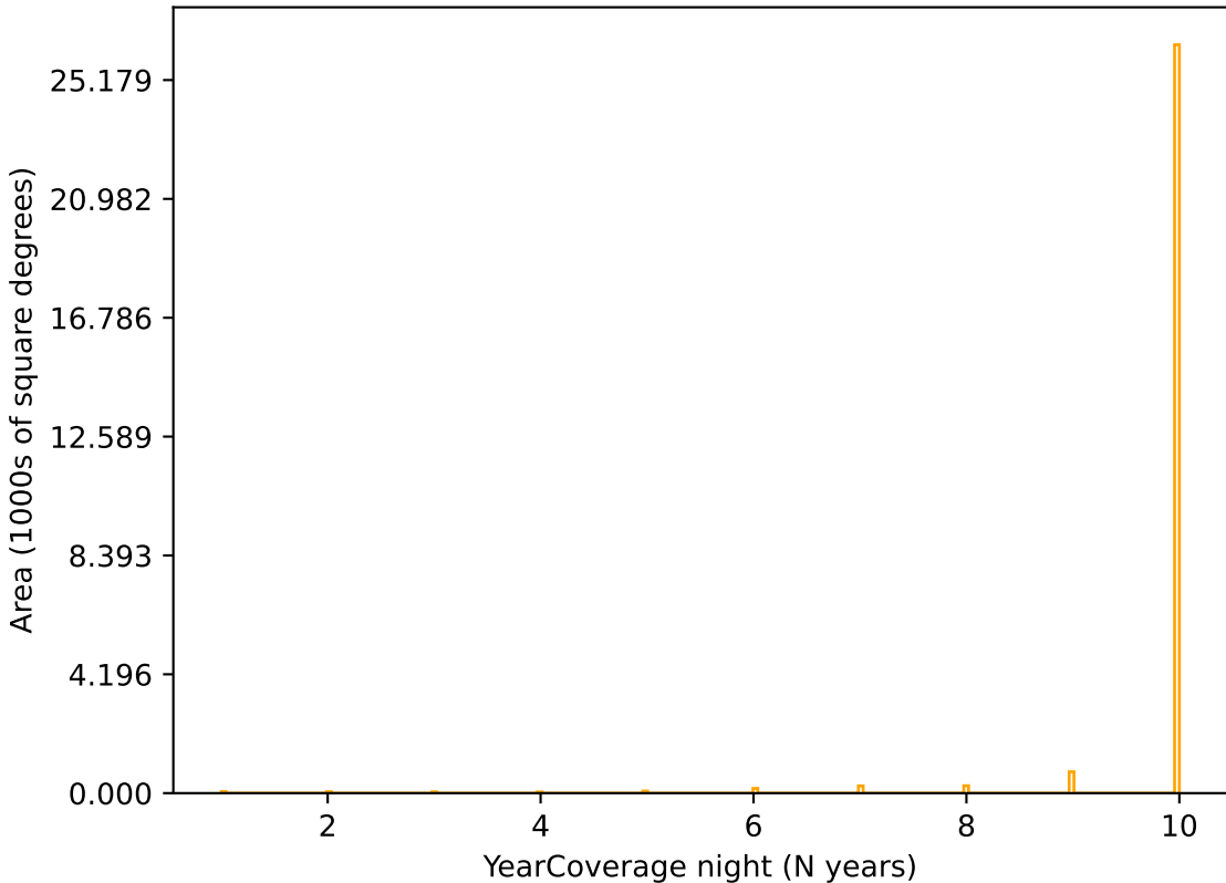
ddf_acor_sf25_lsf30_lsr50_v3.4_10yrs r band: YearCoverage night
