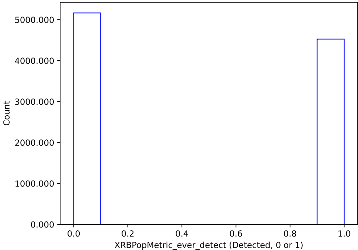
ddf_acor_sf25_lsf30_lsr50_v3.4_10yrs : XRBPoMetric_ever_detect
