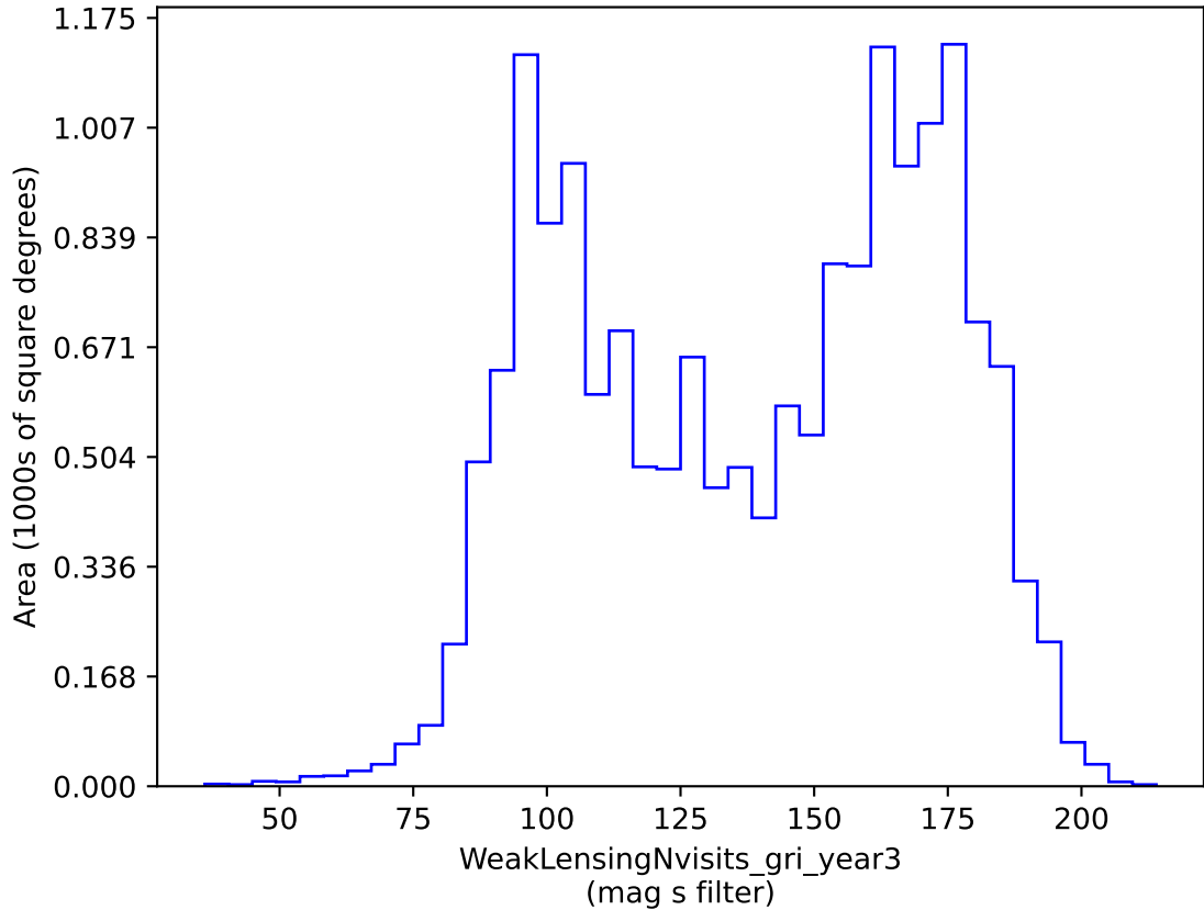
ddf_acor_sf25_lsf30_lsr50_v3.4_10yrs gri band non-DD: WeakLensingNvisits_gri_year3
