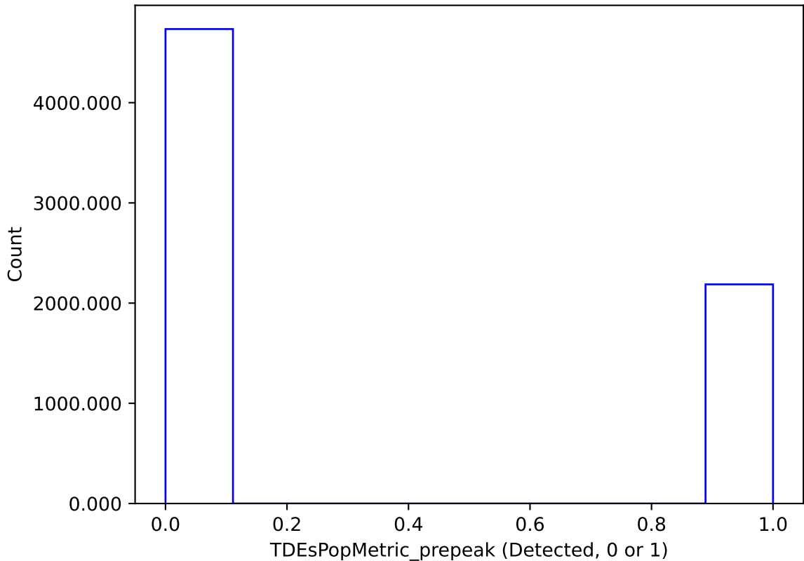
ddf_acor_sf25_lsf30_lsr50_v3.4_10yrs : TDEsPopMetric_prepeak
