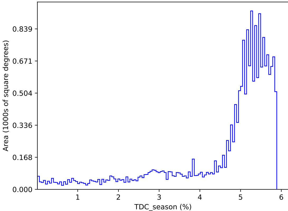
ddf_acor_sf25_lsf30_lsr50_v3.4_10yrs : TDC_season
