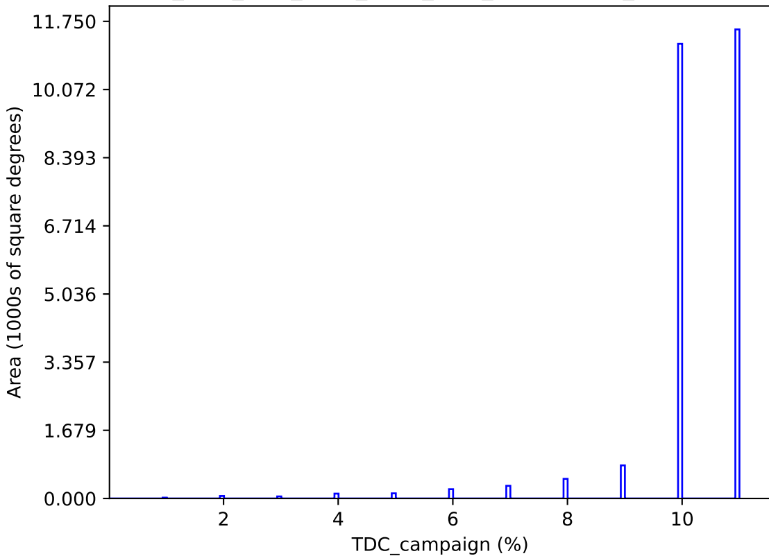
ddf_acor_sf25_lsf30_lsr50_v3.4_10yrs : TDC_campaign
