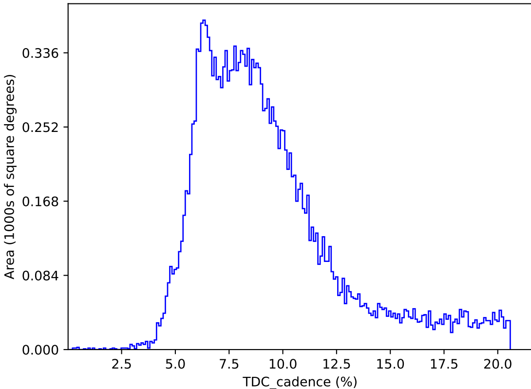
ddf_acor_sf25_lsf30_lsr50_v3.4_10yrs : TDC_cadence
