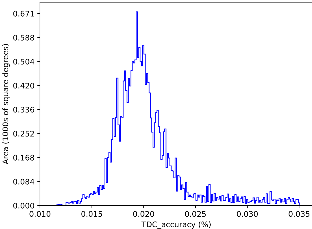
ddf_acor_sf25_lsf30_lsr50_v3.4_10yrs : TDC_accuracy
