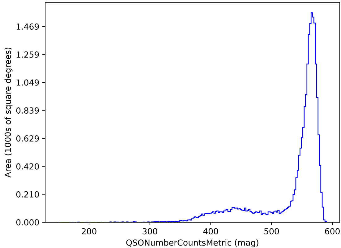
ddf_acor_sf25_lsf30_lsr50_v3.4_10yrs y band and non-DD: QSONumberCountsMetric
