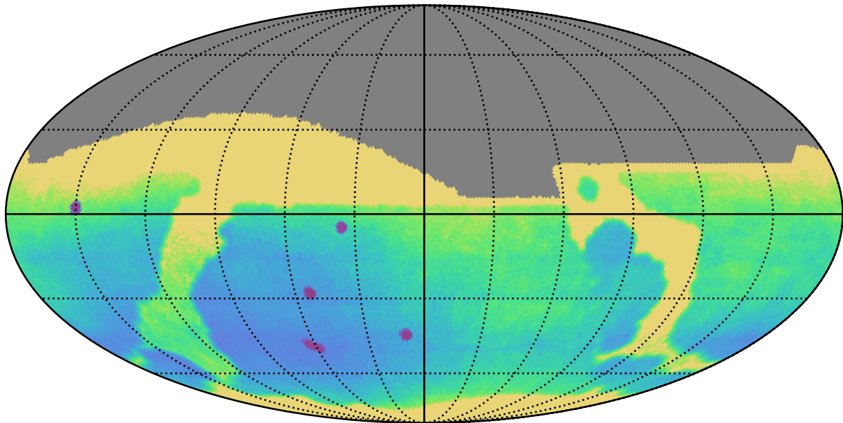
ddf_acor_sf25_lsf30_lsr50_v3.4_10yrs : Parallax Uncert @ 24.0
