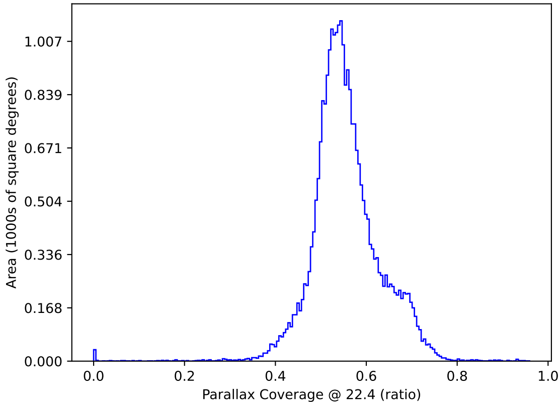
ddf_acor_sf25_lsf30_lsr50_v3.4_10yrs : Parallax Coverage @ 22.4
