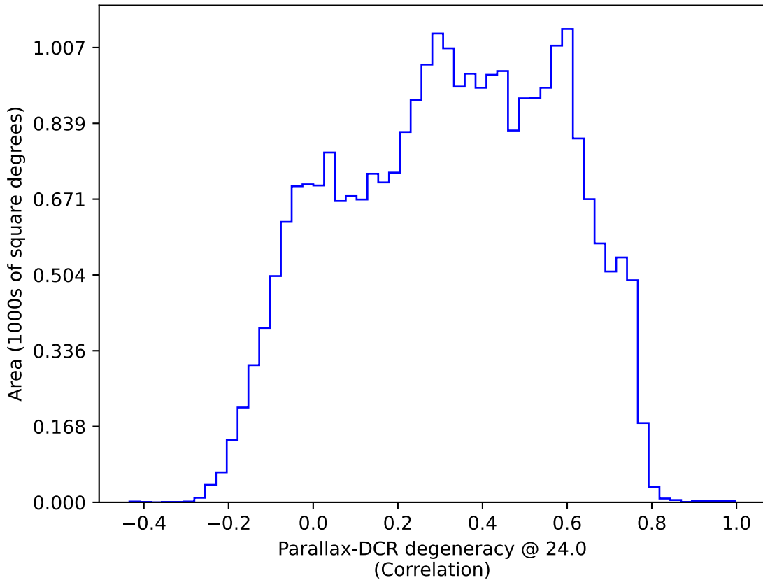
ddf_acor_sf25_ls30_lsr50_v3.4_10yrs : Parallax-DCR degeneracy @ 24.0
