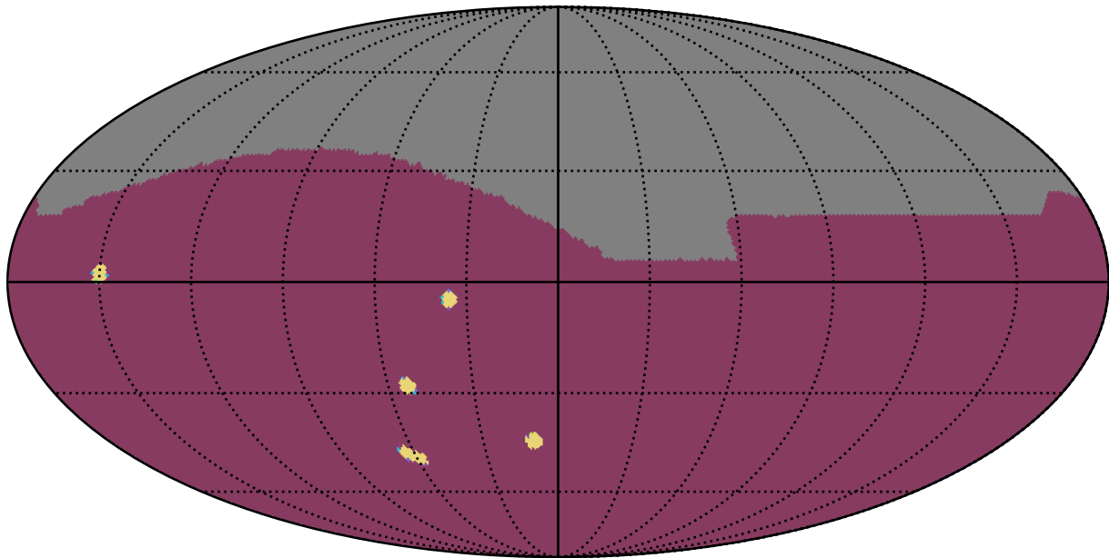
ddf_acor_sf25_lsf30_lsr50_v3.4_10yrs : NumberOfQuickRevisits
