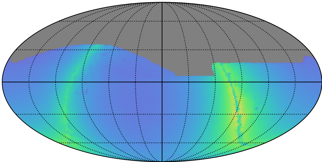
ddf_acor_sf25_lsf30_lsr50_v3.4_10yrs r: Nstars_no_crowding
