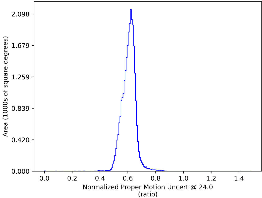
ddf_acor_sf25_lsf30_lsr50_v3.4_10yrs : Normalized Proper Motion Uncert @ 24.0
