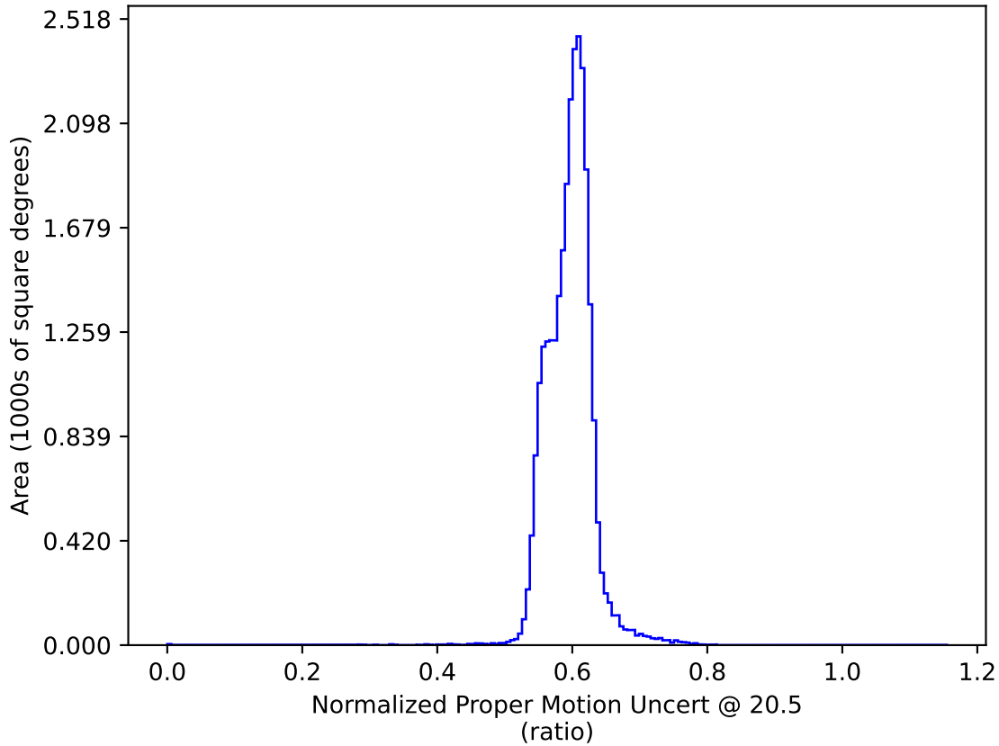
ddf_acor_sf25_lsf30_lsr50_v3.4_10yrs : Normalized Proper Motion Uncert @ 20.5
