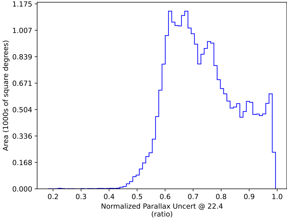
ddf_acor_sf25_lsf30_lsr50_v3.4_10yrs : Normalized Parallax Uncert @ 22.4
