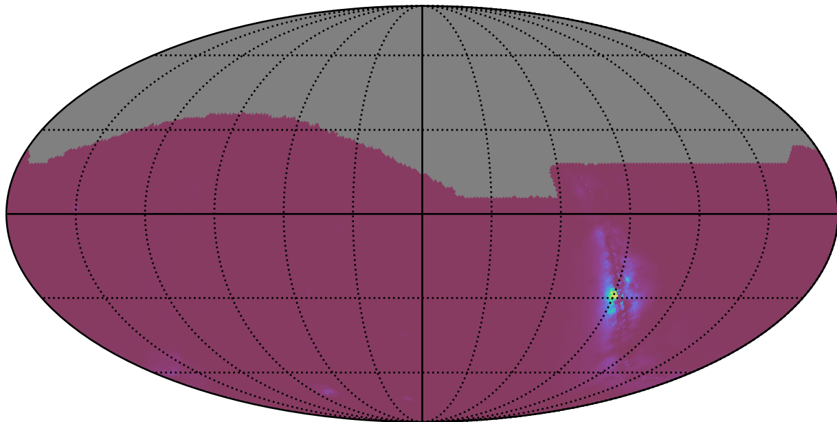
ddf_acor_sf25_lsf30_lsr50_v3.4_10yrs : NlcPoints
